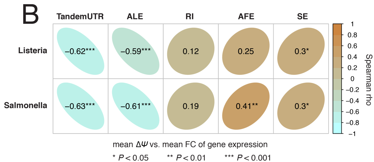
S10 Fig. Inter-individual variation of global shifts in alternative splicing.
