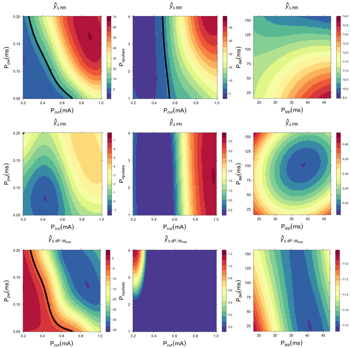
S2 Fig. Example surface responses of the chronotropic, dromotropic and inotropic effects to VNS (respectively the first, second and third rows), generated with a Gaussian process regression for sheep 3
