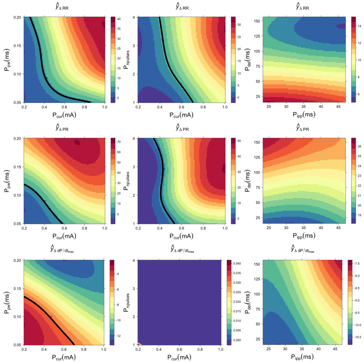
S4 Fig. Example surface responses of the chronotropic, dromotropic and inotropic effects to VNS (respectively the first, second and third rows), generated with a Gaussian process regression for sheep 5
