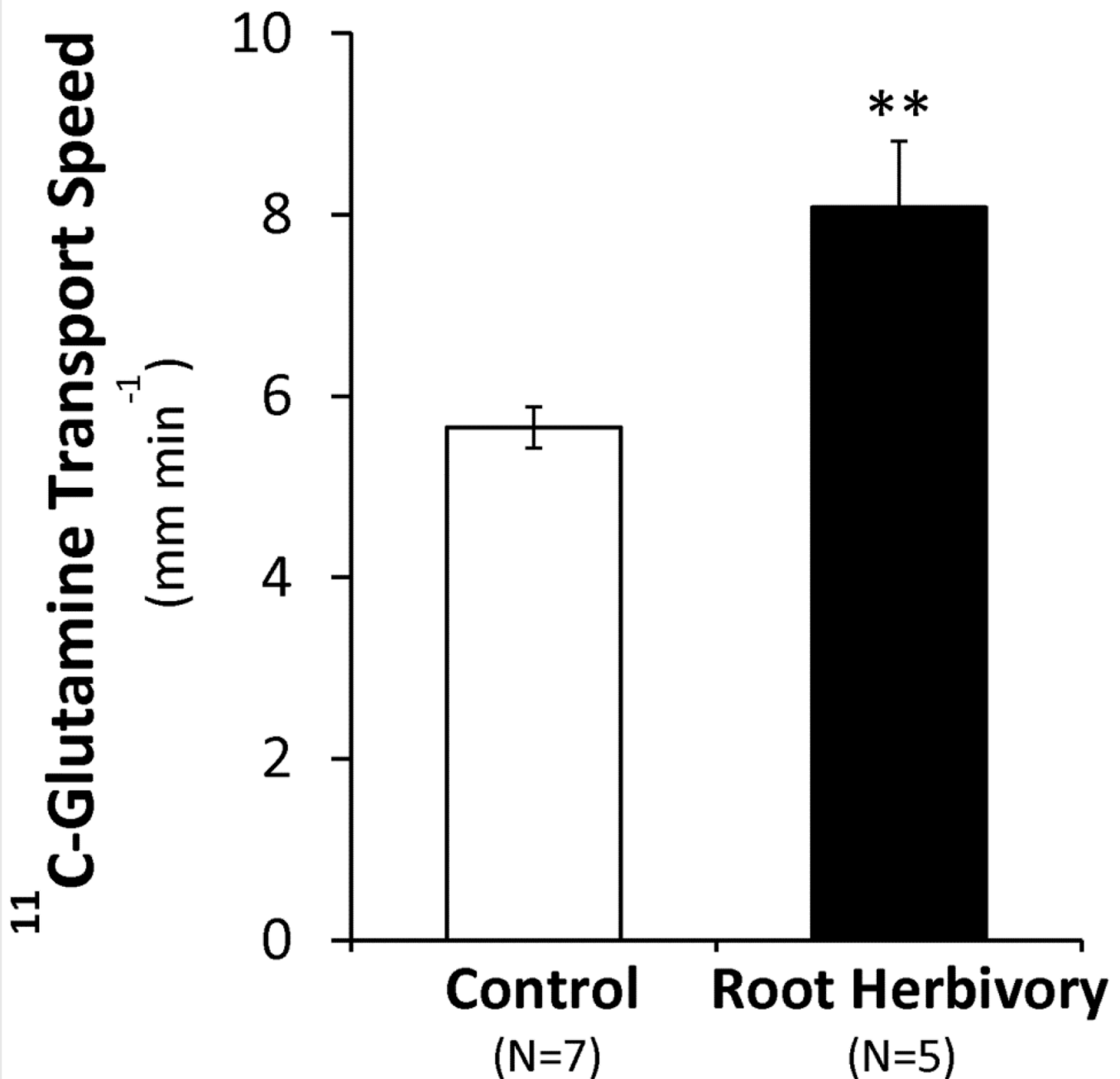
Supplemental Figure 4. Transport speed ( \text{mm min}^{-1} ) of L-[5- ^{11}\text{C} ]glutamine plotted as a function of root herbivore treatment. Statistical significance was denoted as: *, P \leq 0.05 ; **, P \leq 0.01 ; ***, P \leq 0.001 .
