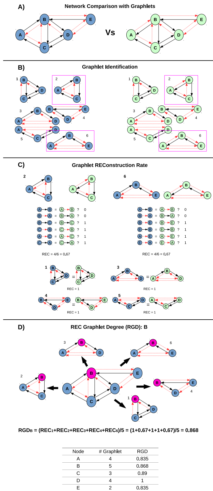
Fig S1: Topological comparison of two small networks
