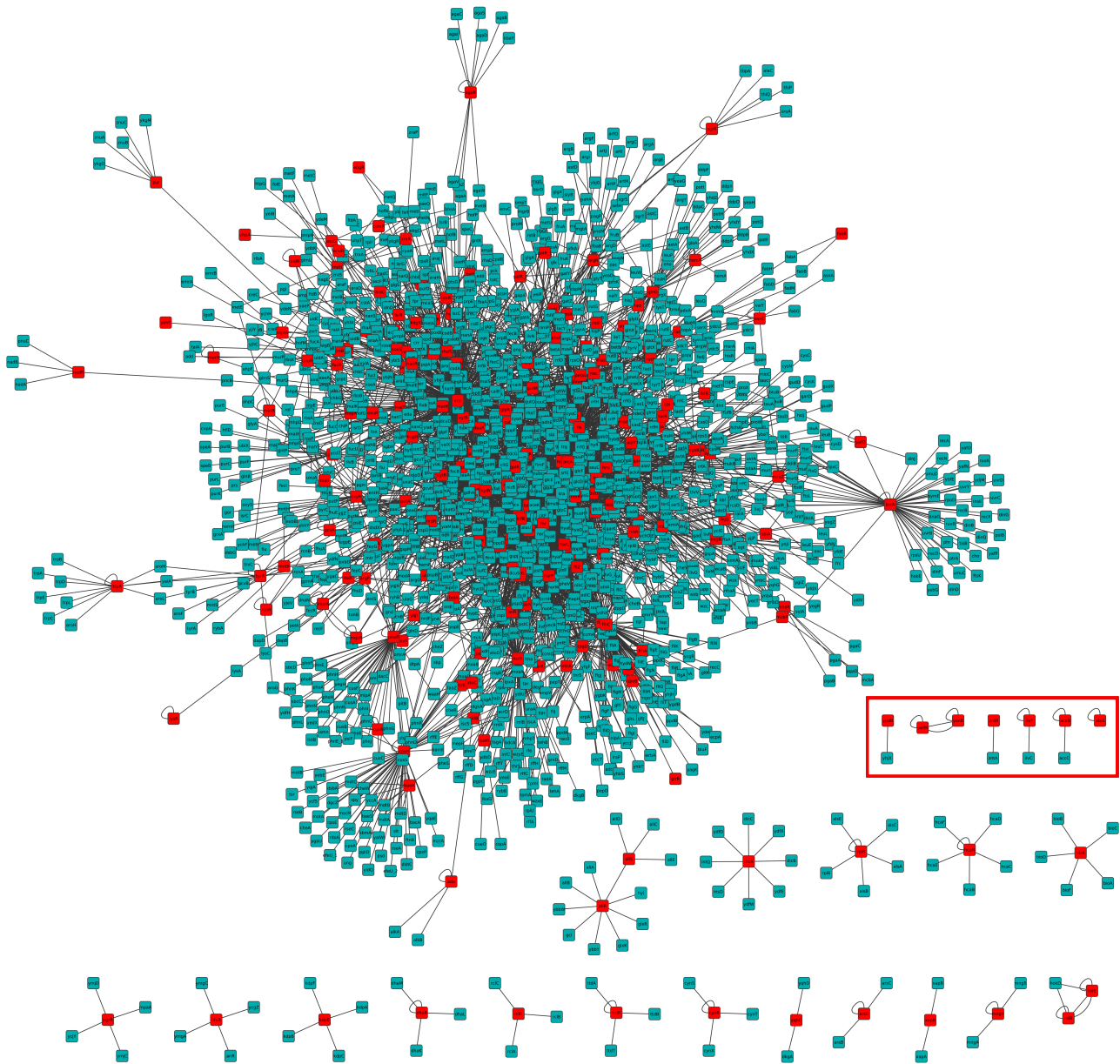
E. coli gold standard network. This image shows visually the gold standard used through the study with different purposes. Transcription Factor encoding genes are colored in red. The eleven nodes that do not form graphlets are shown within a red box.
