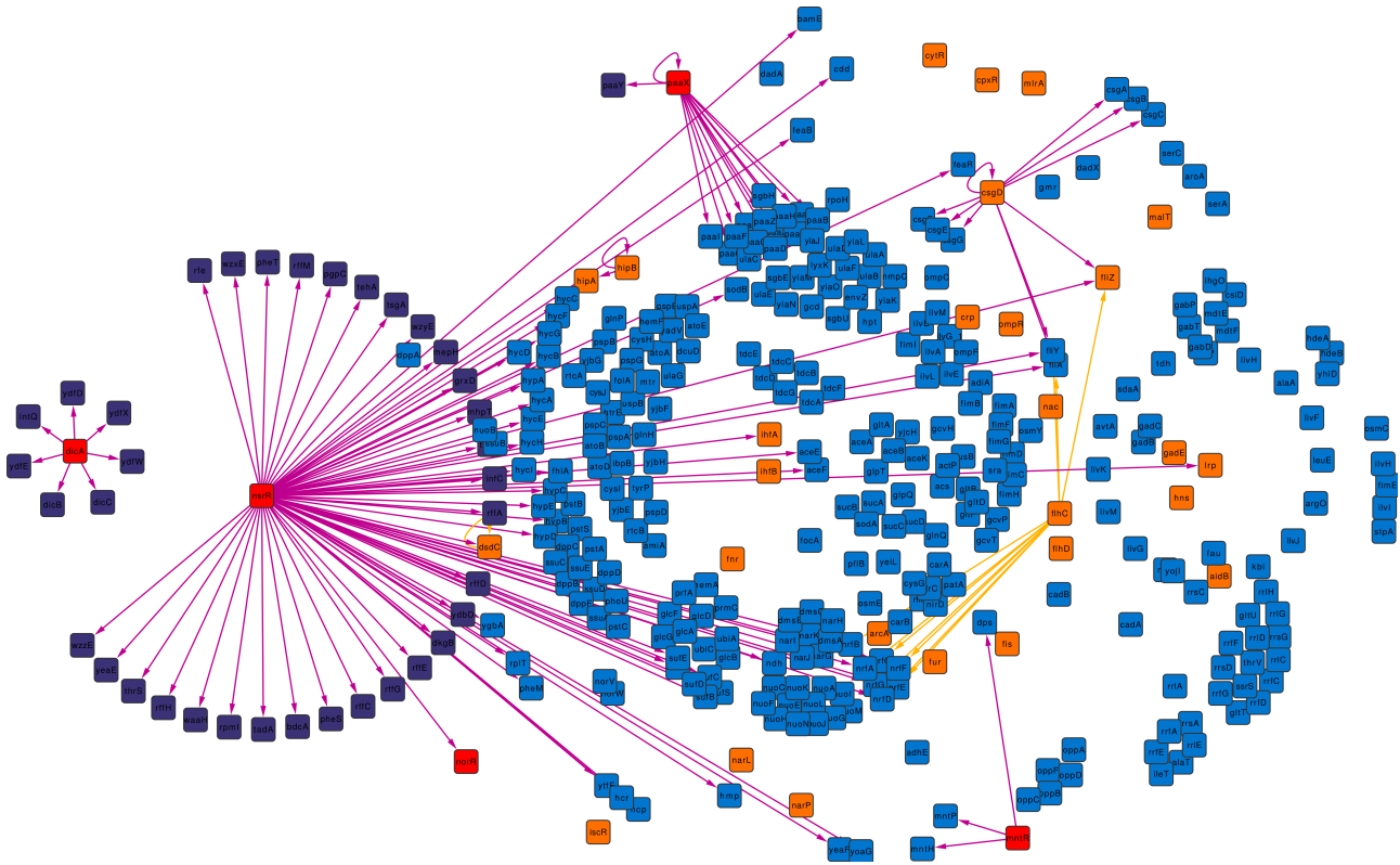
Merged sub-network of the TFs whose RGD varies the most using suspension network at 15 hours as reference. Only FP and FN edges are shown. Color codes are the same as in Figs 4 and 5 in the main text.
