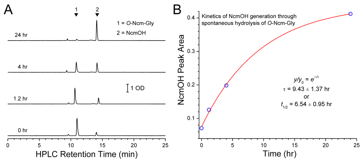
S3 Fig. Spontaneous hydrolysis of O -Ncm-Gly
