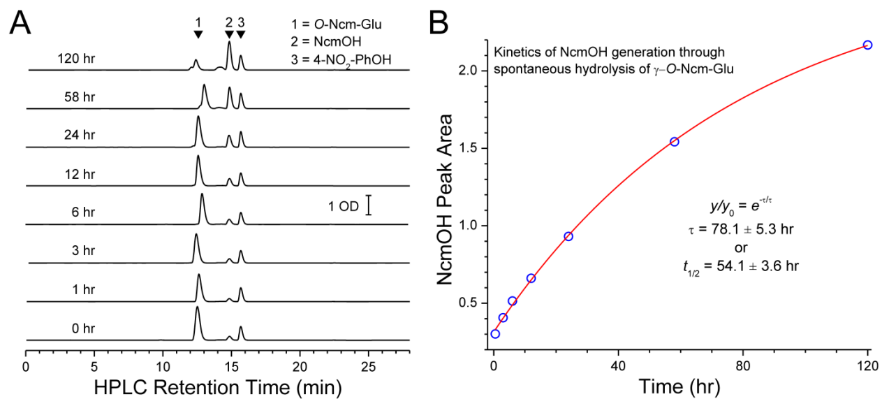
S4 Fig. Spontaneous hydrolysis of \gamma -O-Ncm-Glu
