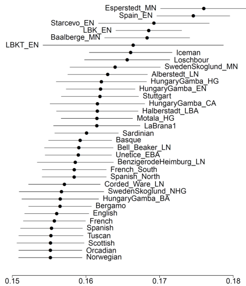
(c) Spain_MN
