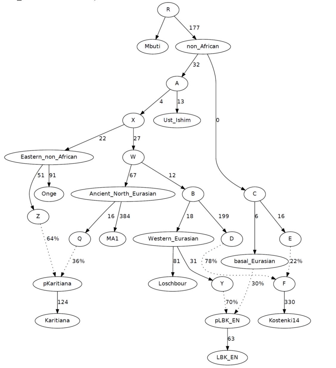
Figure S8.4 Kostenki14 as a 2-way mixture with basal Eurasian admixture like that of the first farmers (however, topologically equivalent to Fig. S8.5 due to 0 drift in non_African→C branch)
