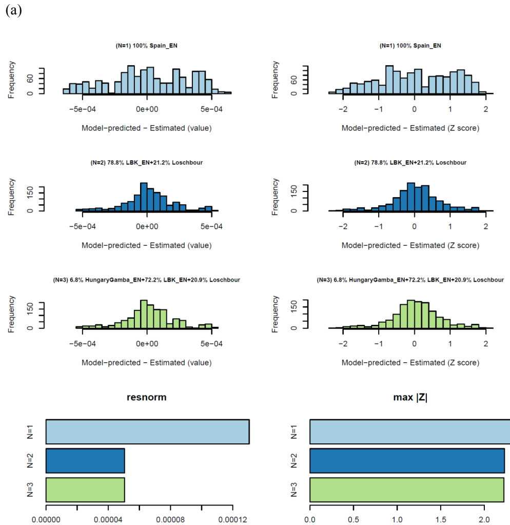
Figure S9.6: Modeling Spain_MN as a mixture of earlier populations. (a) We present in the left column a histogram of raw f_4 -statistic residuals and on the right Z-scores for the best-fitting (lowest resnorm ) model at each N . In the bottom row, we show on the left how resnorm and the maximum |Z| score change for different N . (b) resnorm of different N=2 models.
