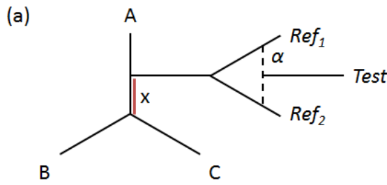
Figure S9.2: Test is a mixture related to two reference populations Ref 1 and Ref 2 . Three possible topologies are shown: (a) Ref 1 and Ref 2 are symmetrically related to A, B, C . (b) Ref 1 and Ref 2 are differentially related to one outgroup A , and symmetrically related to the other two B, C . (c) Ref 1 and Ref 2 are related to two of the outgroups A, C and symmetrically related to the third B . In case (a) all f_4 -statistics involving Test , Ref 1 , Ref 2 are identical and cannot be used to estimate mixture proportions. In cases (b, c) f_4 -statistics involving Test are a weighted average of those involving Ref 1 and Ref 2 .
