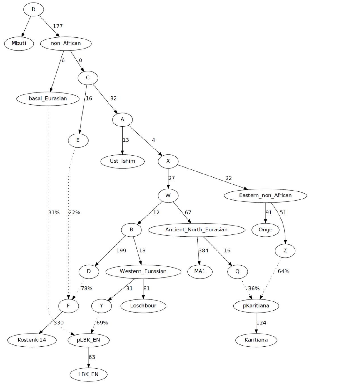
Figure S8.5 Kostenki14 as a 2-way mixture with basal Eurasian admixture after that of the first farmers (but topologically equivalent to Fig. S8.4 due to 0 drift in non_African→C branch).
