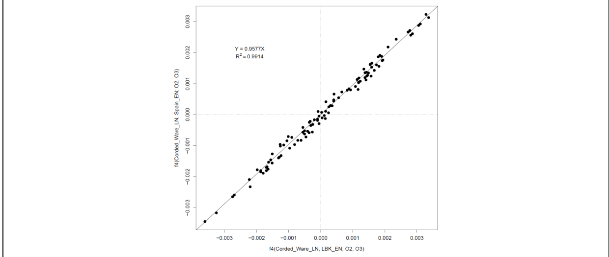
Figure S9.13: When the two references are a clade with respect to the Test (as Spain_EN and LBK_EN are with respect to Corded_Ware_LN), a line with positive slope is observed.
