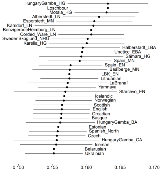
(b) Bell_Beaker_LN
