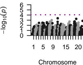
PH, No-imputed
