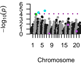
TKW, No-imputed
