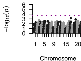
PH, RF
