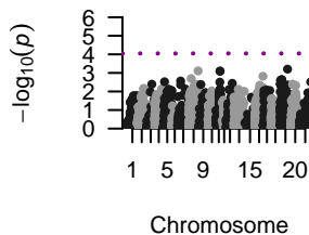
PH, Mean
