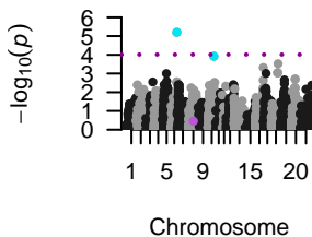
SPM, MVN-EM
