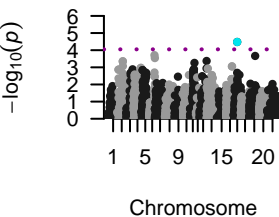
DH, No-imputed
