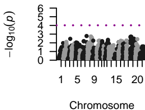
PH, MVN-EM
