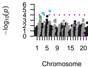
TKW, MVN-EM
