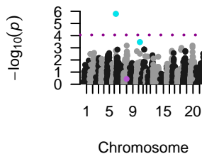
SPM, Mean
