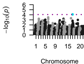
DH, Mean
