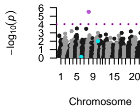
SPM, RF
