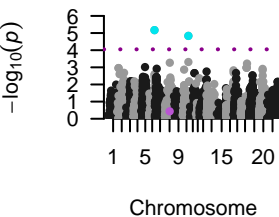
SPM, No-imputed
