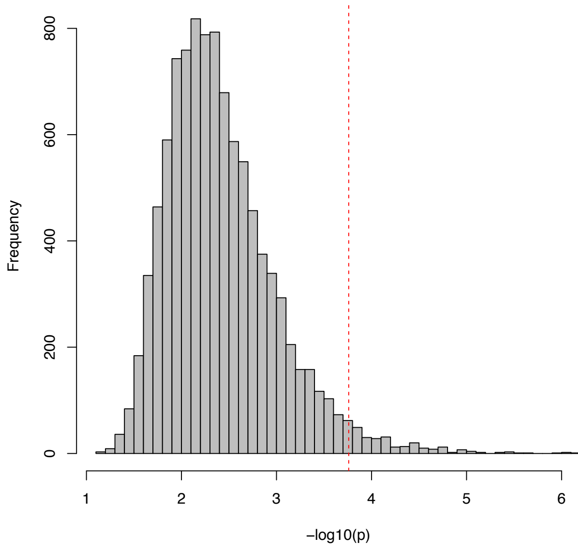
Distribution of permuted minimum p-values
