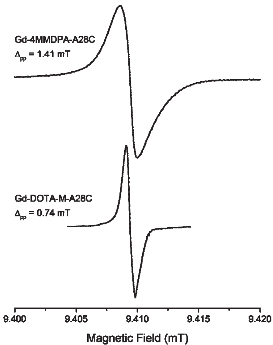
Figure S4. Cw EPR spectra of frozen DNP-solutions of Gd-4MMDPA-labeled and Gd-DOTA-M-labeled A28C mutant of ubiquitin measured at a \mu\text{w} frequency of 263 GHz and a temperature of 100 K. \Delta_{pp} is the peak-to-peak linewidth of the cw spectra ( i.e. , first derivative of the absorption spectra).
