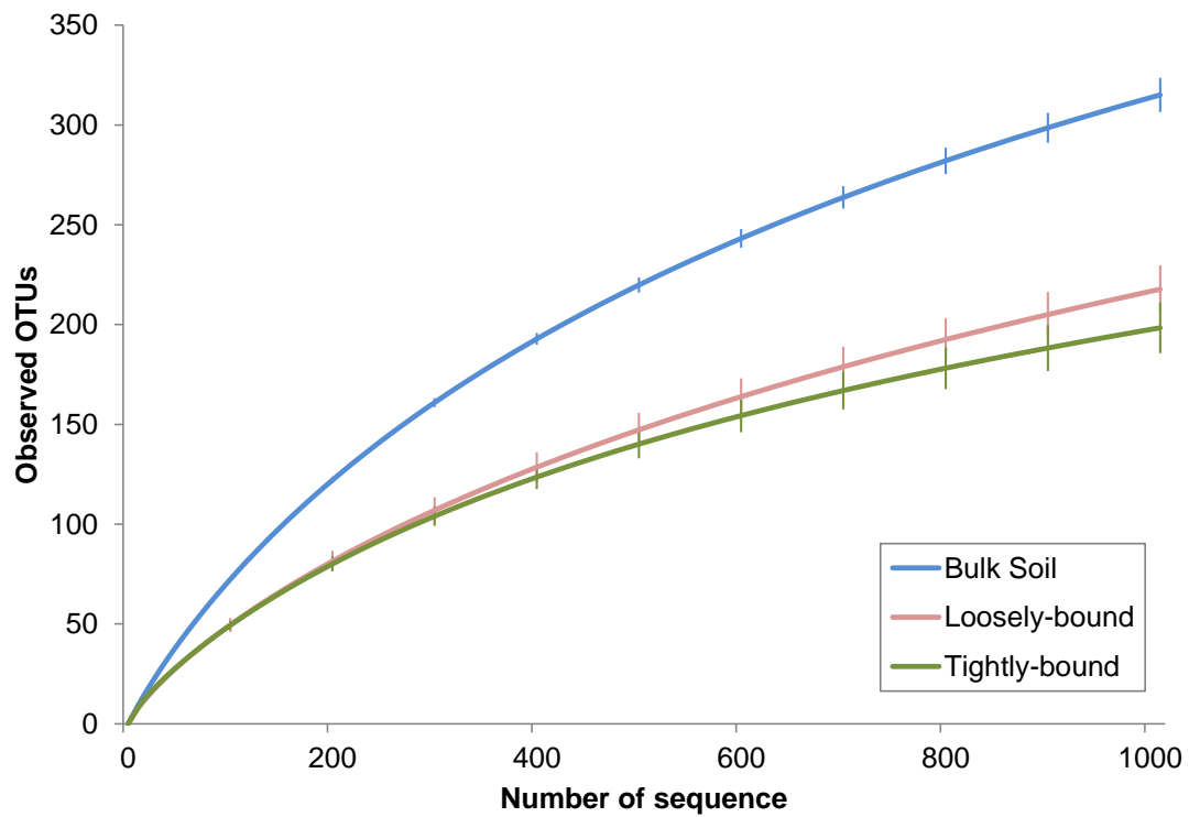
S4 Fig. Rarefaction curves of bacterial OTUs identified in the bulk soil and Brachypodium rhizospheres. Bacterial community was analyzed with 16S pyrosequencing, and 1015 sequences were randomly subsampled from each sample to achieve even sequencing depth. Means are shown \pm SE (n=4-5).
