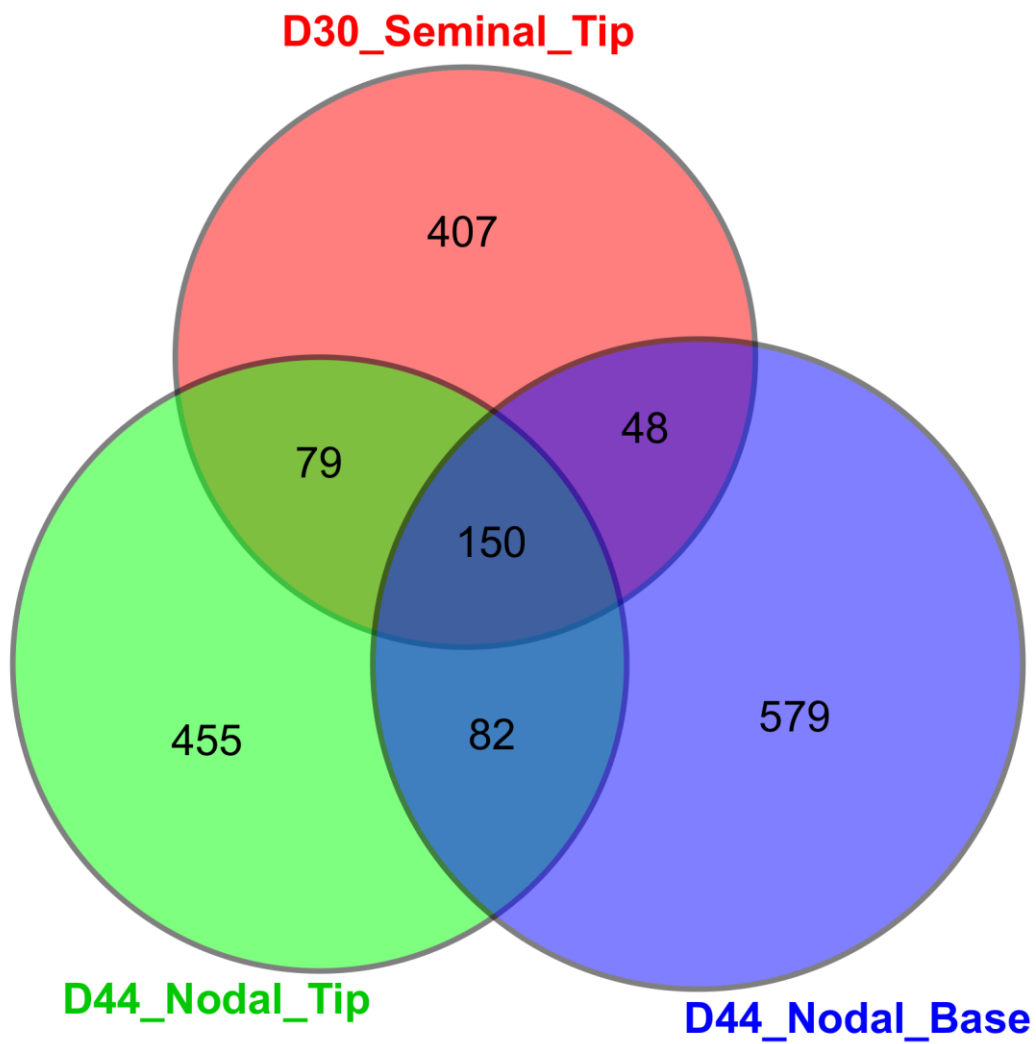
S9 Fig. Venn diagram showing the number of shared and unique bacterial OTUs identified in Brachypodium seminal and nodal root systems. An OTU was considered unique if it was present in at least one replicate of one group, and absent in the other groups (n=8-9).
