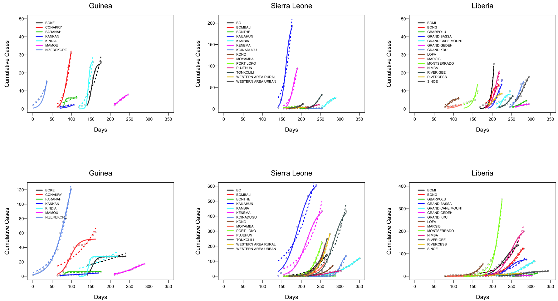
Figure S2. Exponential (dashed lines) and logistic (solid lines) fits to the weekly cumulative time series (model in equations 1 and 3 respectively) for all three countries at the subnational level. Using data from the first 6 weeks (upper panel) and 15 weeks (lower panel) of the outbreak in each region.
