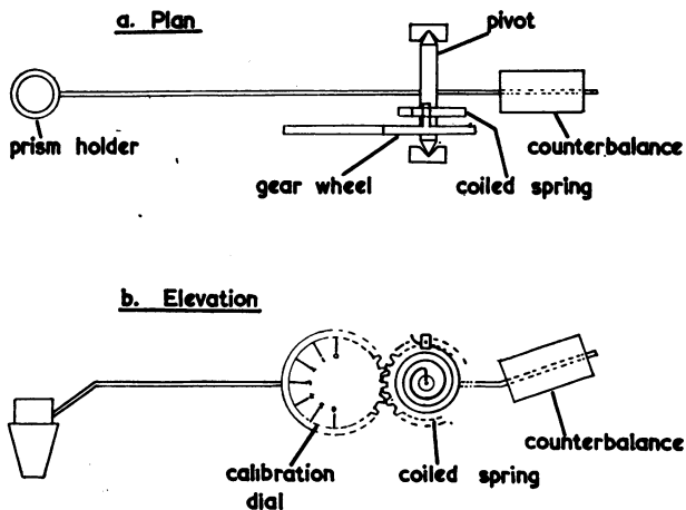
FIG. 1.—Diagram of mechanism: (a) plan, (b) elevation.
