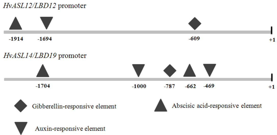
Fig. S1 Promoter analysis of HvASL12/LBD12 and HvASL14/LBD19 genes
