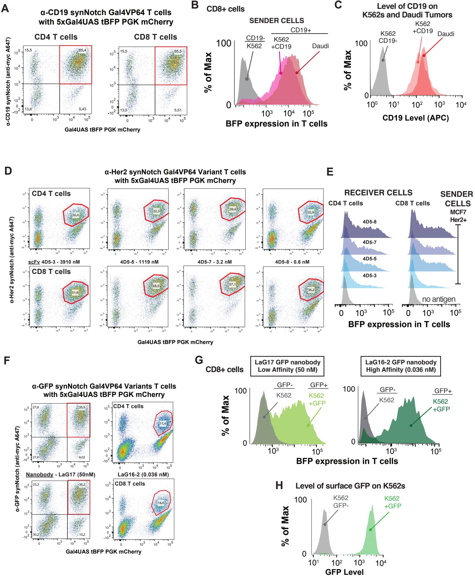
Fig S1. synNotch Receptors Drive Antigen-dependent Custom Gene Regulation in Primary Human T cells (related to main text Figure 1).
