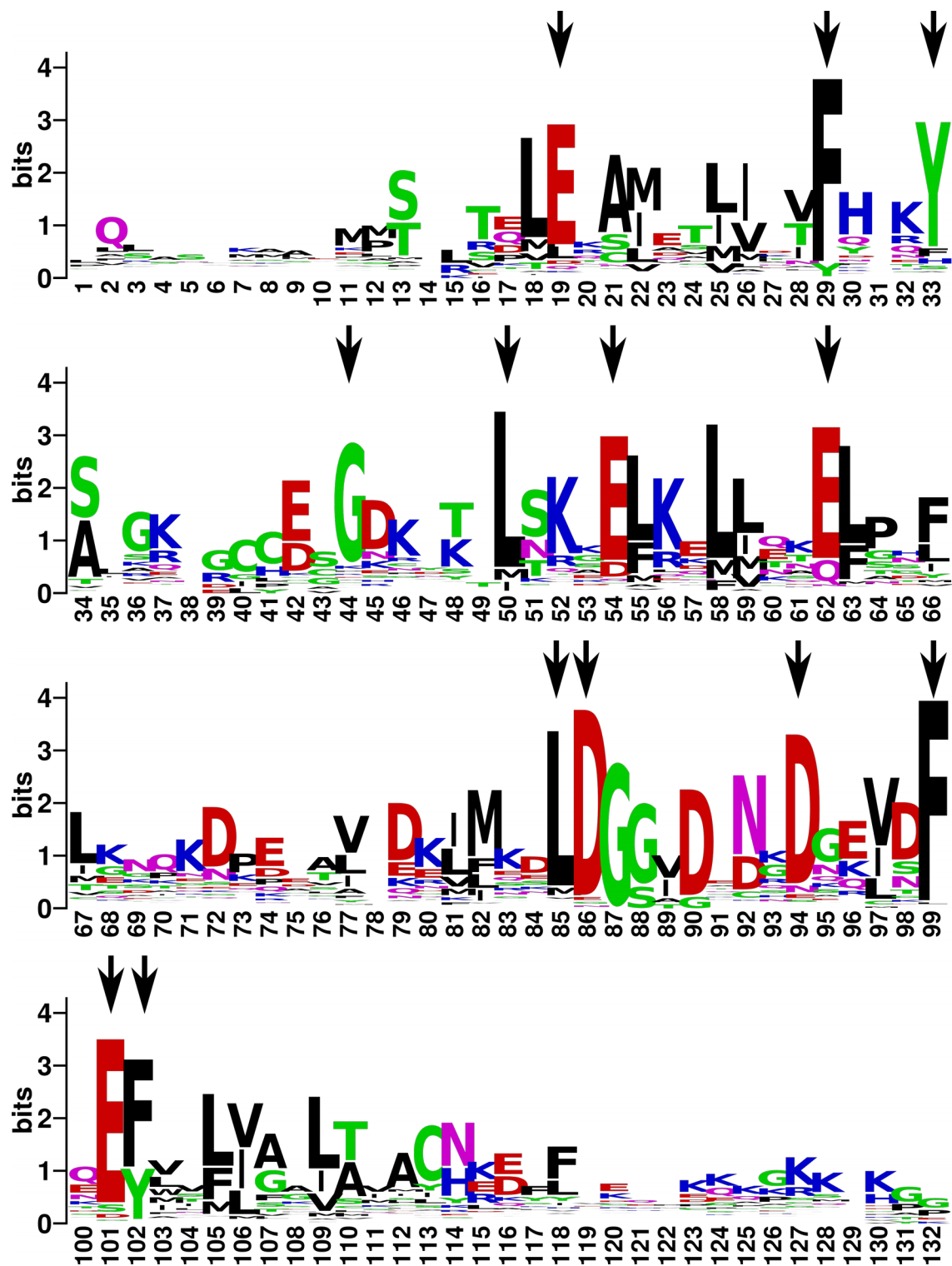
S1 Fig: Sequence logo of alignment of S100 proteins. Sequence logo indicates relative occurrence of amino acids at each position in the alignment. Taller letters indicate higher frequency at that position. Arrows indicate 13 key residues we used to verify/anchor the alignment.
