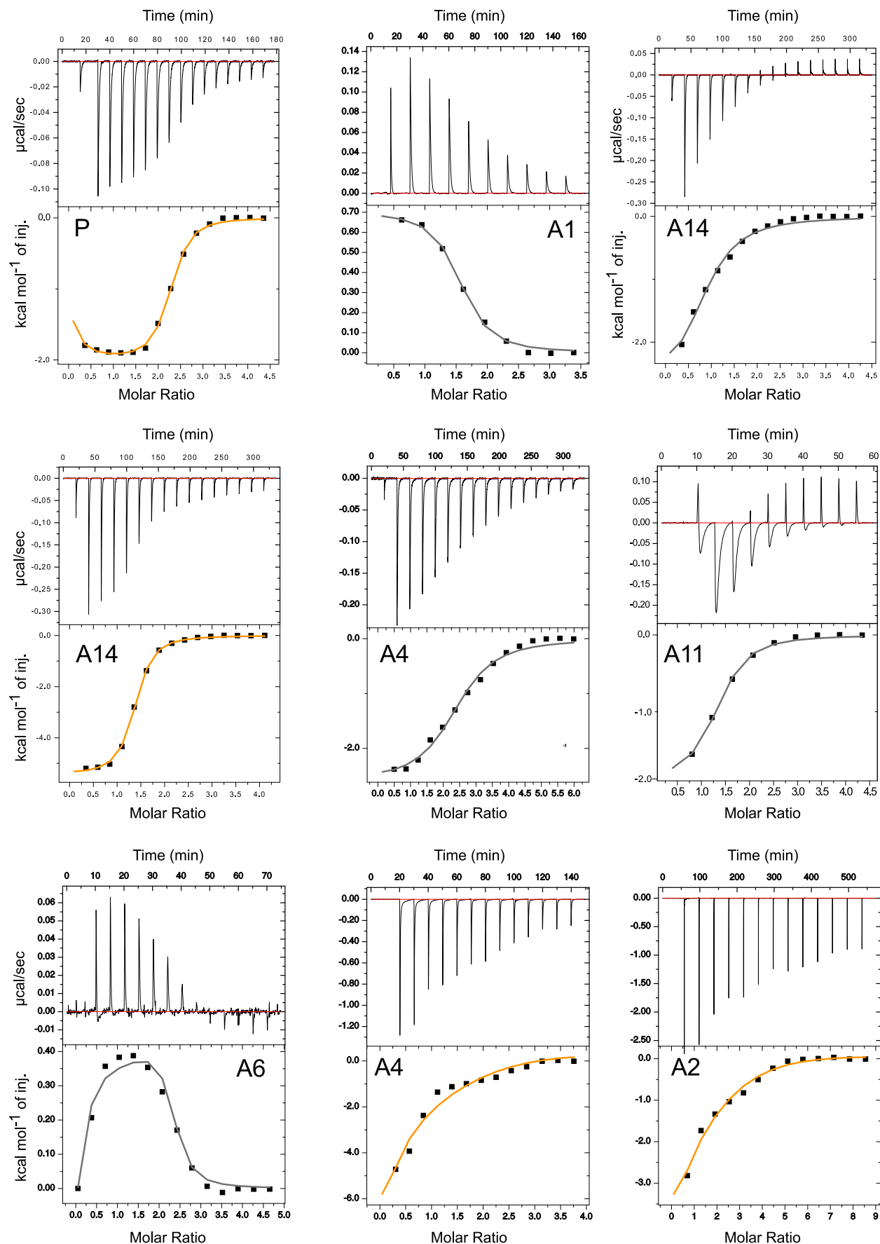
S4 Fig: Example ITC traces for various S100 proteins. Each panel is a single human ortholog, indicated by the name on the graph. Color of fit indicates metal used as titrant: \text{Zn}^{2+} (gray) or \text{Cu}^{2+} (copper). Top sub-panel for each panel is a raw power vs. time curve. Bottom sub-panel for each panel is integrated heat versus molar ratio. The model fit is denoted by the heavy line through the fit points.
