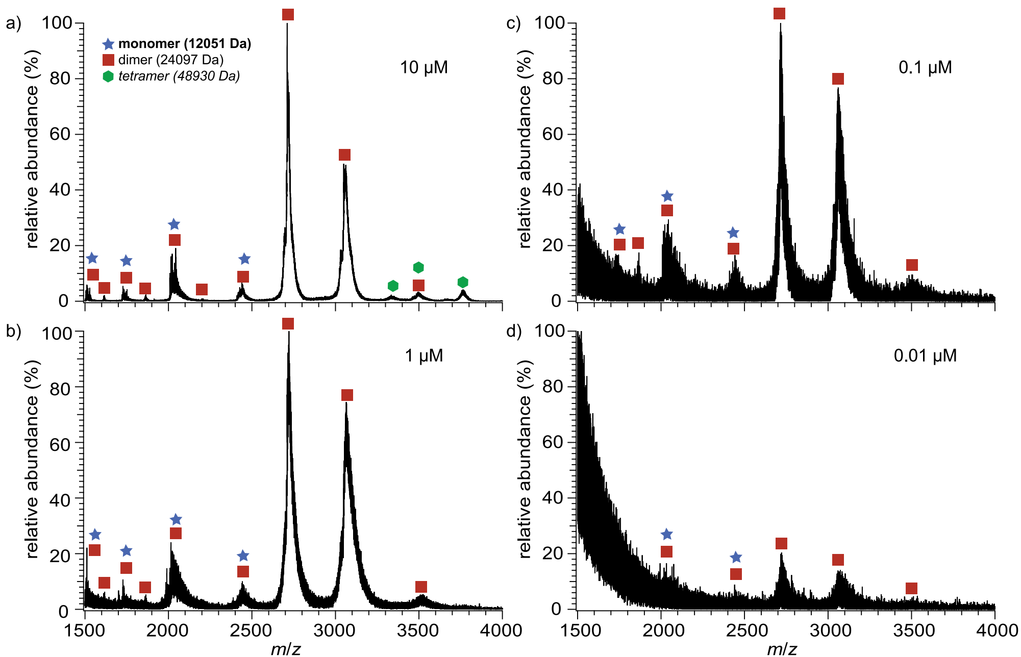
S7 Fig tunB dilution by ESI-MS. tunB mass spectra at concentrations of a) 10 \mu\text{M} , b) 1 \mu\text{M} , c) 0.1 \mu\text{M} , and d) 0.01 \mu\text{M} demonstrate that tunB homodimers are robust to dilution, indicating that this is a specific interaction. Homotetramer is observed only in the most concentrated sample, thus homotetramer signal likely arises from non-specific interactions during the electrospray process.
