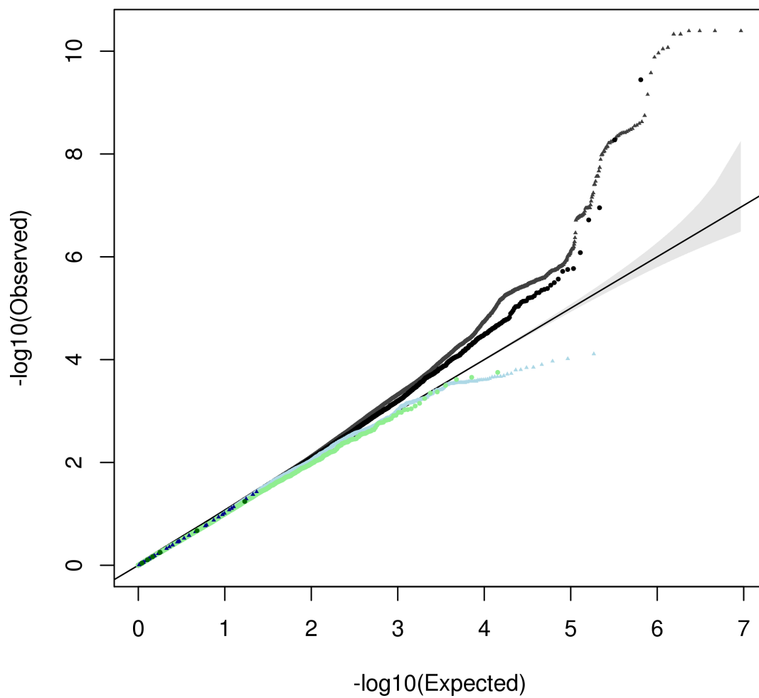
S1 Fig. QQ-plot for GERA non-Hispanic whites. Previously-identified sub-threshold SNPs are separated from the rest of the SNPs (dark green is the SNP itself, light green is within 0.5Mb of the SNP). Typed SNPs are circles, imputed are triangles.
