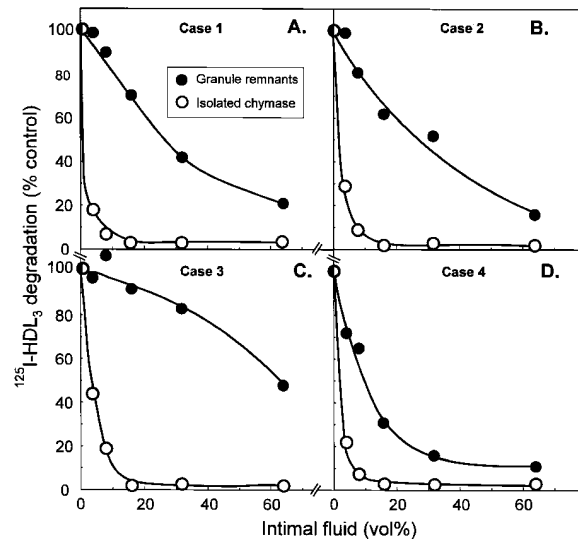
Figure 7. Degradation of HDL 3 by mast cell granule remnants or isolated chymase in the presence of extracellular fluid obtained from human aortic intima. 125 I-HDL 3 (0.6 mg/ml, 0.5 cpm/ng) was incubated at 37°C for 2 h in 20 \mu l of a mixture comprising 150 mM NaCl, 1 mM EDTA, and 5 mM Tris-HCl, pH 7.4, with granule remnants (10 \mu g; 17 BTEE units) or isolated chymase (17 BTEE units) in the presence of 4, 8, 16, 32 and 64% (vol/vol) of intimal fluid obtained from four aortic samples. After incubation, the amounts of TCA-soluble 125 I radioactivity were determined, calculated as percents of the 125 I-HDL 3 degradation in the absence of intimal fluid (control), and plotted as a function of inhibitor concentration. In the different cases, the control values (100%) for granule remnants and isolated chymase, respectively, were 8 and 11% (case 1), 9 and 12% (case 2), 13 and 22% (case 3), and 14 and 23% (case 4) of the total 125 I radioactivity in HDL 3 .
