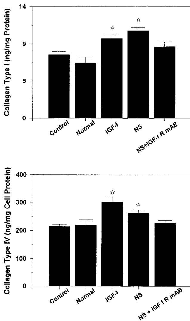
Figure 6. Effect of rhIGF-I (2 nM) and normal or nephrotic (NS) rat urine extract (1:5) in the absence or presence of IGF-I-receptor neutralizing antibody (IGF-I R mAb) on secreted collagen type I (top) and type IV (bottom). Cells were incubated for 60 h. Media were concentrated tenfold and then analyzed by ELISA. Data are mean \pm SEM ( n = 12 per group). * P < 0.05 vs control.
