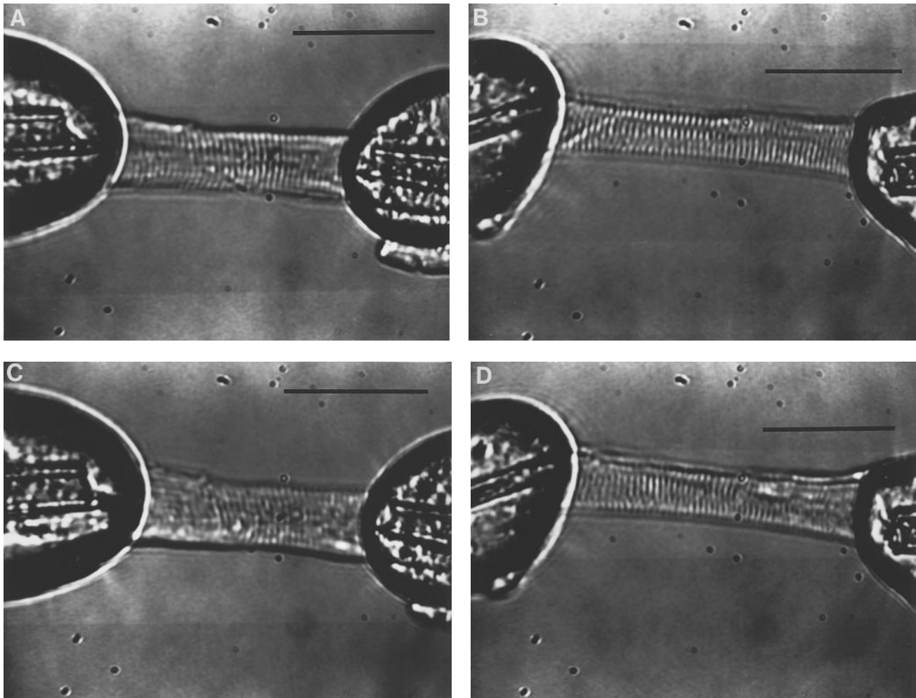
Figure 1. Photomicrographs of representative myocyte-sized myofibrillar preparations from a donor ventricle ( A and C ) and a cardiomyopathic ventricle ( B and D ). Preparations are shown in relaxing solution ( [Ca^{2+}] = 10^{-9} M, A and B ) and maximally activating solution ( [Ca^{2+}] = 10^{-4.5} M, C and D ), and demonstrate preserved striation resolution and minimal shortening of central sarcomeres with maximal activation. Scale bars equal 50 \mu m.
