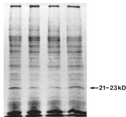
Figure 2. An autofluorograph depicting the inhibition of the carboxyl methylation of a 21–23-kD protein by AFC in intact pancreatic islets. Normal rat islets (groups of 200–250) were preincubated in an isotonic medium in a Krebs-Ringer bicarbonate medium (at 37°C for 4 h) with [ ^3 H-methyl]methionine (50 \mu Ci/ml) to label endogenous SAM pools (19). Cycloheximide (5 \mu M) and actinomycin D (2 \mu M) were added 1 h before provision of labeled methionine in order to inhibit the synthetic incorporation of [ ^3 H]methionine into new proteins. Labeling was carried out for 4 h followed by a 30-min incubation in the presence or absence of either AFC or AGC (100 \mu M each). Labeled proteins were separated by SDS-PAGE (12% acrylamide) and identified by autofluorography. Results are representative of three independent experiments with similar results.
