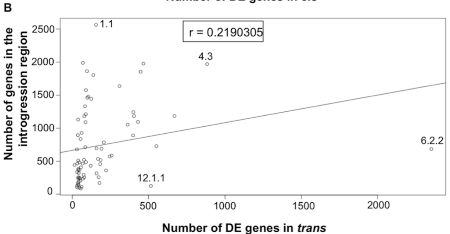
Supplemental Figure S1. Number of genes in the introgression region for an IL and the number of differentially expressed genes at the transcript level compared to cv. M82.
