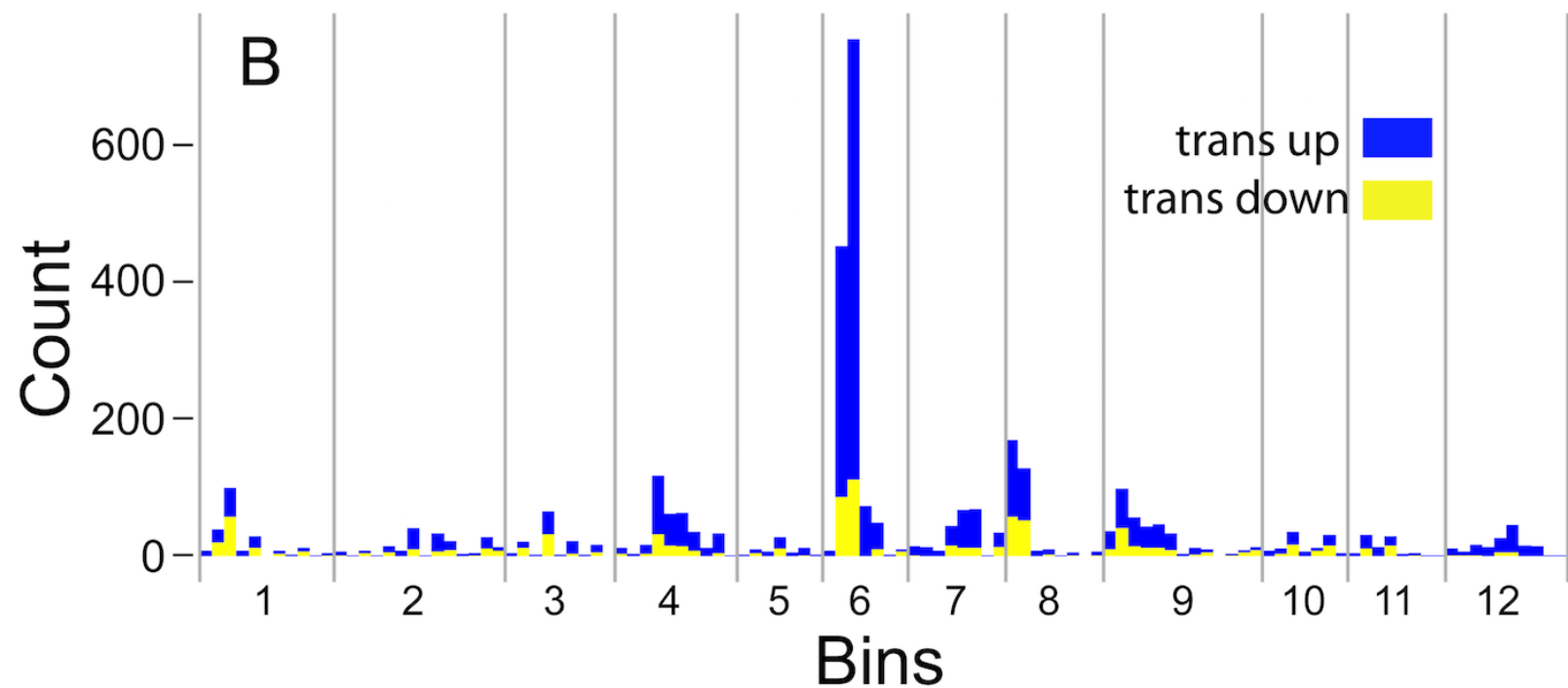
Supplemental Figure S4. Cis - and Trans -eQTL. Histograms plotting the numbers of significant eQTL mapped to each bin across the 12 chromosomes of S. lycopersicum (M82). A. cis -eQTL. B. trans -eQTL.
