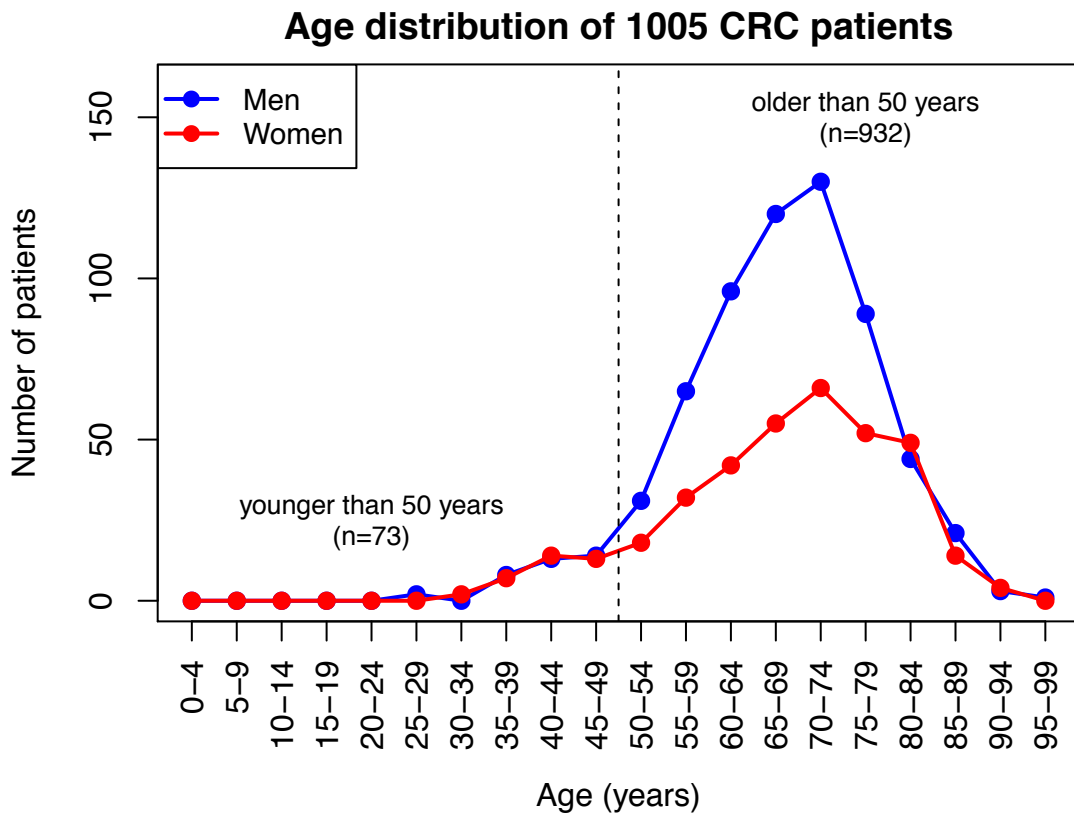
Figure S1. Age distribution of the CRC patients in the 1,005 cases consecutive series recruited for this work. Blue line: men. Red line: women. Seventy three patients were younger than 50 years (left of the dashed line), and 932 patients were older than 50 years.
