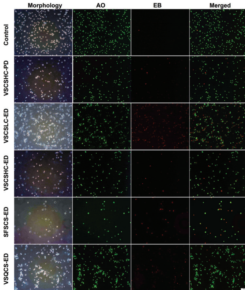
SUPPLEMENTARY FIG. S4. Typical phase and fluorescence micrographs (before and after merging the red and green channels) corresponding to that shown in Figure 4C.
