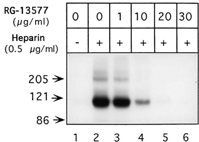
Figure 4. RG-13577 inhibits heparin-mediated FGF-2-receptor cross-linking and dimerization. Confluent HS-deficient CHO-pgsA745-flg cells were incubated (2 h, 4°C) with 1 ng/ml ^{125}\text{I} -FGF-2 in the absence (lane 1) or presence (lanes 2–6) of 0.5 \mu\text{g/ml} heparin and increasing concentrations (1–30 \mu\text{g/ml} ) of RG-13577 (lanes 3–6). Unbound ^{125}\text{I} -FGF-2 was removed and the cells were washed (3 \times ). The cells were then incubated with 0.3 mM DSS, quenched with 150 mM glycine, 2 mM EDTA, lysed, and subjected to a 7.5% SDS-PAGE and autoradiography, as described in Methods. Molecular weight markers are in kilodaltons.
