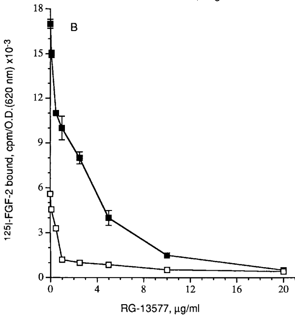
Figure 2. RG-13577 inhibits FGF-2 binding to FGFR-1. (A) Soluble receptor binding: FRAP-conditioned medium was incubated (2 h, 4°C) with ^{125}\text{I} -FGF-2 in the presence of increasing concentrations of heparin (○) or RG-13577 (□). FRAP-conditioned medium was also incubated with increasing concentrations of RG-13577 in presence of 20 ng/ml heparin (●). The bound FRAP-FGF-2 complexes were immunoprecipitated with anti-alkaline phosphatase monoclonal antibodies coupled to Sepharose, followed by washing with PBS. ^{125}\text{I} -FGF-2 receptor binding was determined by counting the tubes in a gamma counter. Each data point represents the mean \pm SD of triplicate samples. The dashed line represents FGF-2 receptor binding activity in presence of 20 ng/ml heparin. Any activity above this line indicates a synergistic effect of RG-13577, while points below the line represent an inhibitory effect. (B) Cell-surface receptor binding: CHO-pgsA-745-flg cells were incubated (2 h, 4°C) with 1 ng/ml ^{125}\text{I} -FGF-2, with or without increasing concentrations of RG-13577, in the absence (□) or presence of 200 ng/ml heparin (■). The amount of radioactivity specifically bound to high-affinity binding sites was determined as described in Methods. Each data point represents the mean \pm SD of four culture wells.
