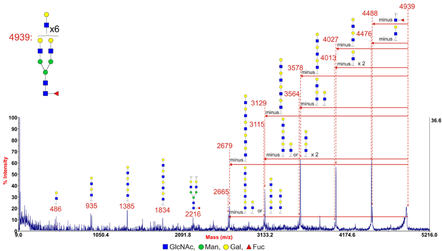
Fig. S5. Annotated MALDI-TOF MS spectrum of permethylated sialidase S digested N-glycan at 4939 from CTB. Data were acquired in the form of [M+Na]^+ ions. Peaks were annotated with putative fragment ions according to the molecular weight.
