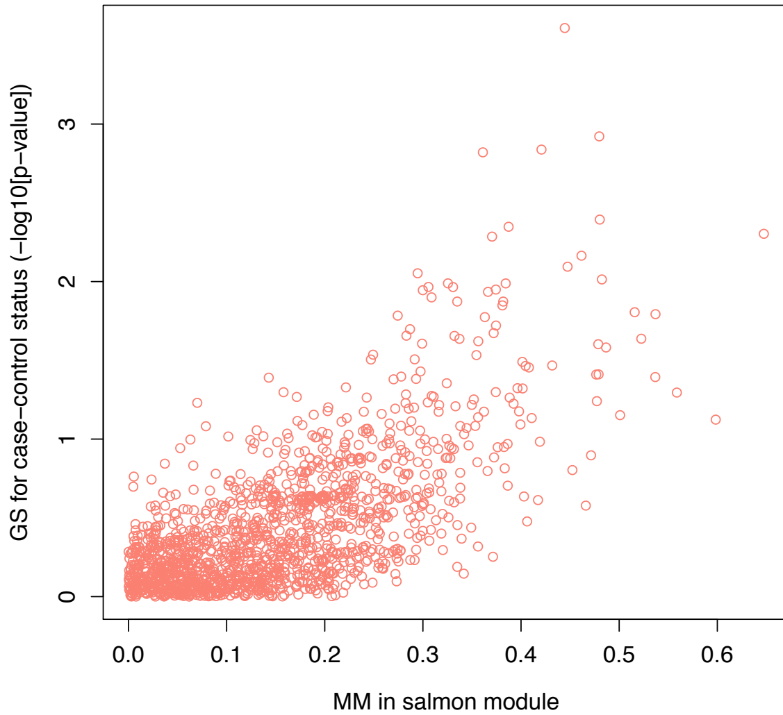
Module membership vs gene significance cor=0.69, p<1e-200
