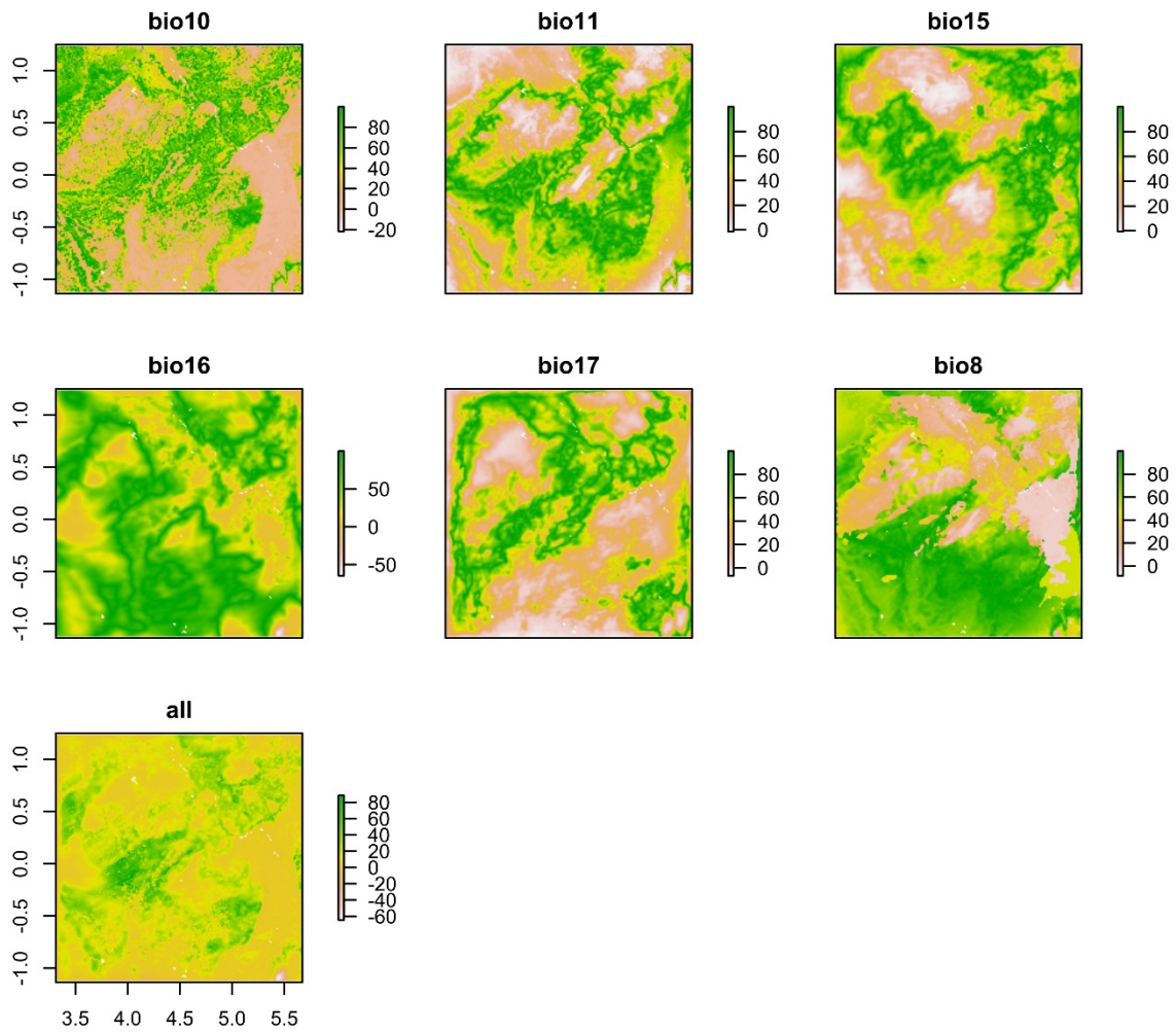
S3 Fig D. BIO MCP 150 MESS maps.
