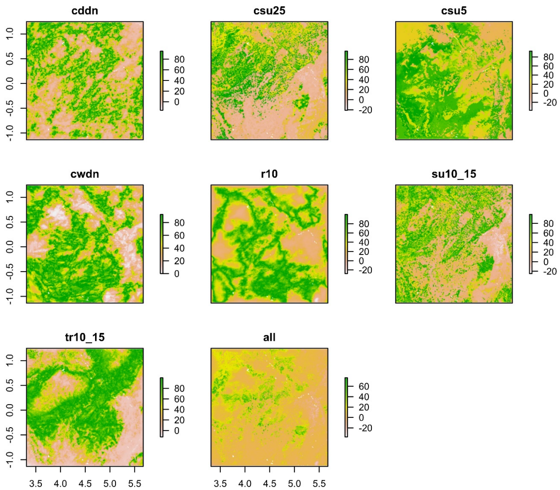
S3 Fig A. ECA MCP 70 MESS maps.
