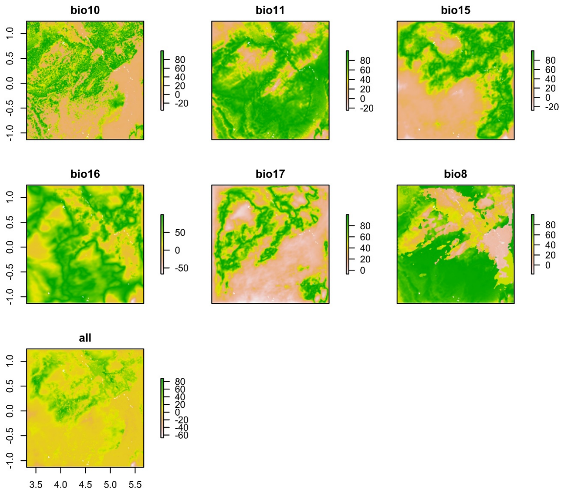
S3 Fig C. BIO MCP 70 MESS maps.
