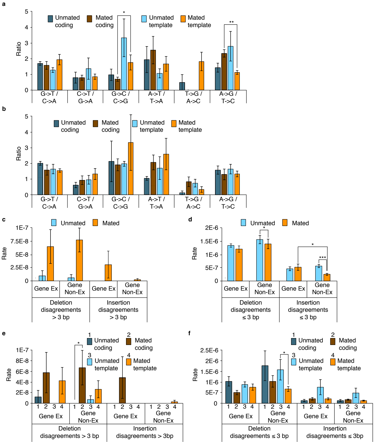
Supplemental Fig S14. Breakdown of duplex disagreement ratios or rates as a function of thresholded gene expression status, strand type, and by disagreement length.
