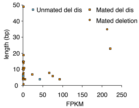
Supplemental Fig S15. Gene duplex deletion disagreements longer than 3 bp and all deletion mutation lengths as a function of gene expression levels and mating status.
