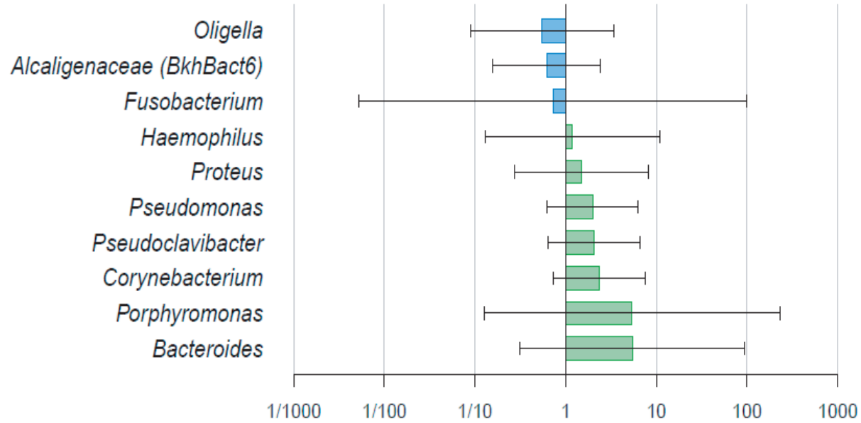
Top 10 Most Abundant Genus in Middle Ear
