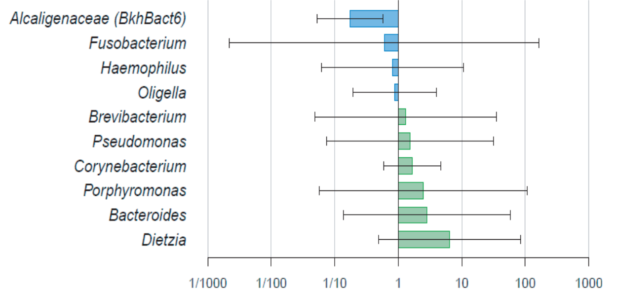
Top 10 Most Abundant Genus in Outer Ear
