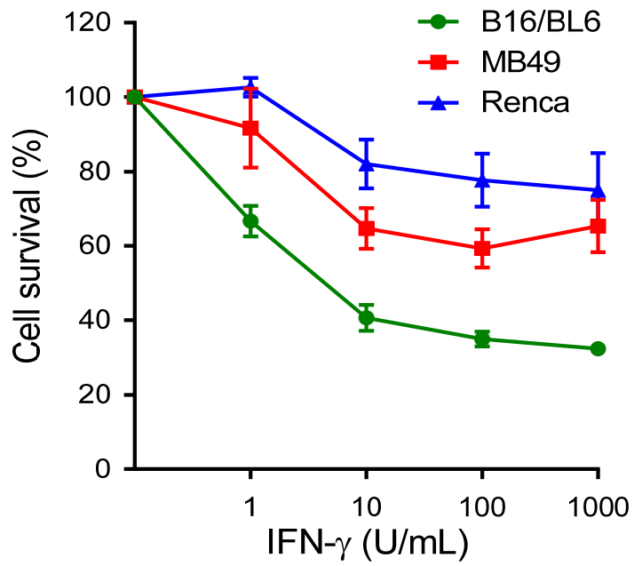
Figure S4. Responsiveness of mouse cancer cell lines B16/BL6, MB49, and Renca to IFN- \gamma treatment, related to Figure 3. Tumor cells treated with varying concentrations of IFN- \gamma for 48 h were assessed for their survivals.
