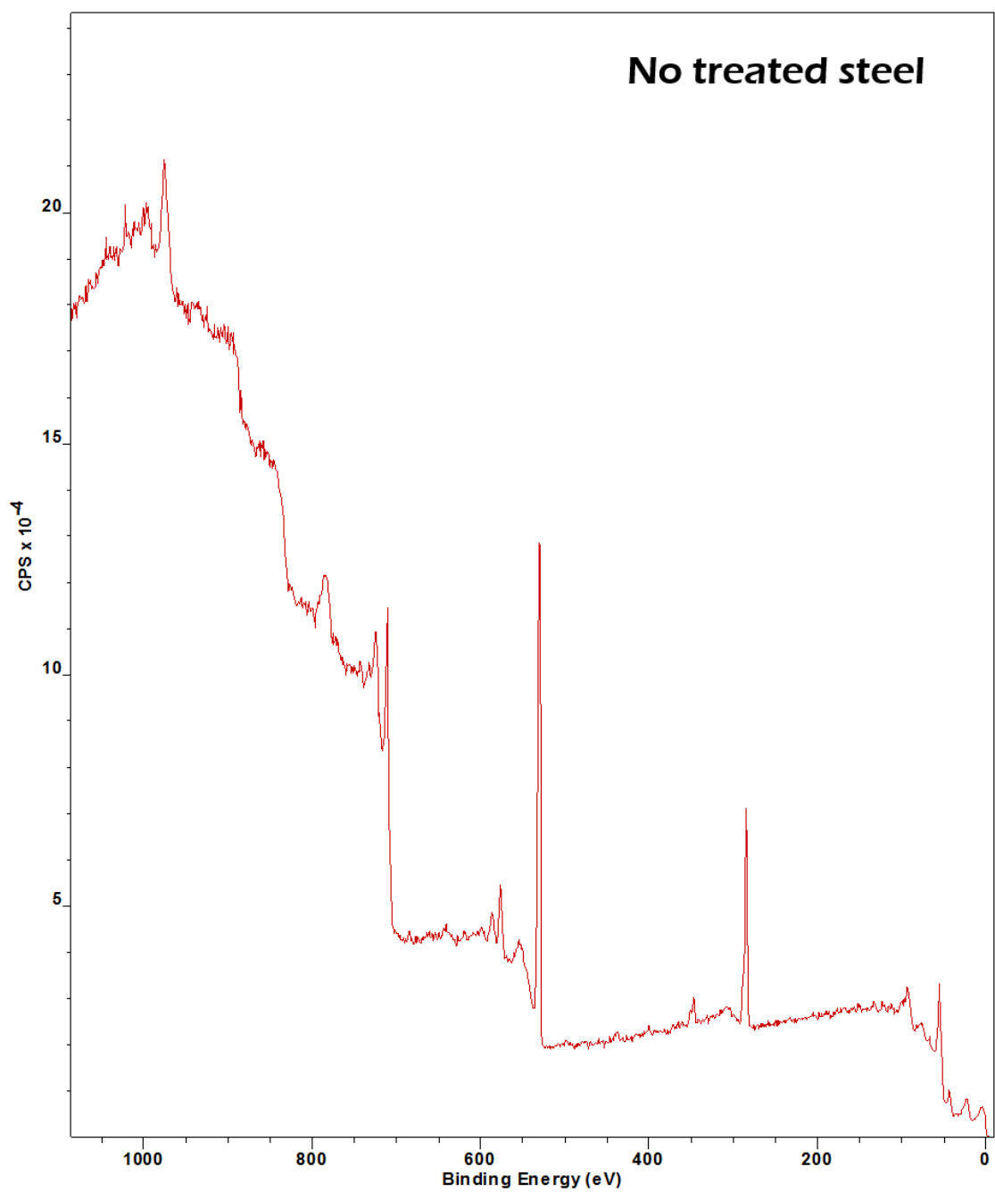
Figure S2. XPS Spectra corresponding to the no treated areas of the steel.
