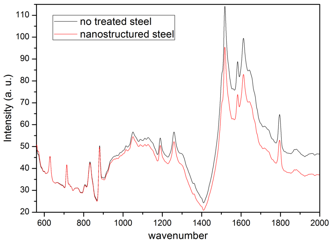
Figure S1. FTIR Spectra corresponding to the no treated areas (black line) and to the nanostructured areas with LIPSS (red line).
