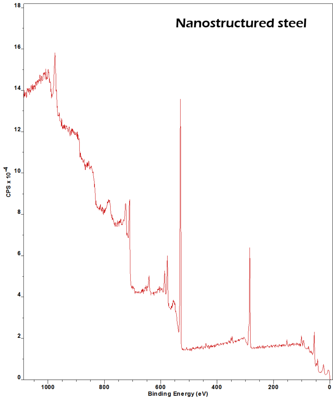
Figure S3. XPS Spectra corresponding to the nanostructured areas of the steel.
