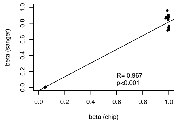
0% and 100% methylated CpGs
