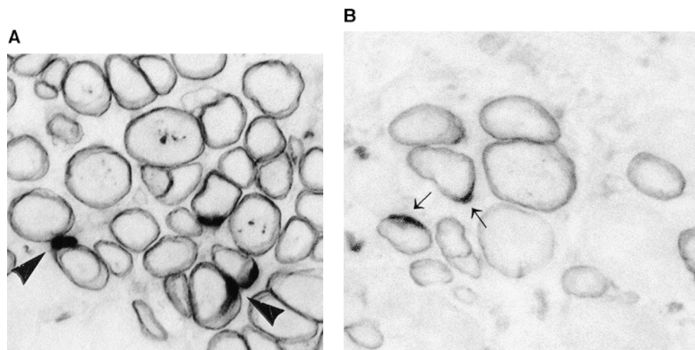
Figure 3. 8- \mu m sections of tibialis anterior reacted for acetylcholinesterase activity and labeled with human \beta -spectrin antibody from (A) mouse injected with normal myoblasts and (B) from mouse injected with NARP myoblasts. The intensely stained areas at the edge of the fibers represent motor end plates (arrows), suggesting that the regenerated human fibers are innervated. \times 115 .
