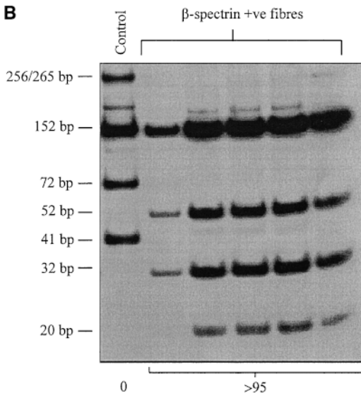
Figure 5. Restriction enzyme digest analysis for quantification of mutant mtDNA in MERRF myoblasts (A). When the MERRF mutation is present, the 72-bp fragment is cut into 52 and 20 bp. A nonpathological, homoplasmic mtDNA, 9-bp deletion within the amplified region is shown by the presence of a 32-bp fragment in the DNA from the patient rather than the 41-bp fragment seen in the control DNA. Also shown is DNA from a subject with the 9-bp deletion who does not possess the MERRF mutation. The level of mutant mtDNA is represented as percentages underneath. (B) \beta -spectrin positive fibers from the tibialis anterior of a mouse injected with MERRF myoblasts. The mutant load (represented as percentages underneath) is similar to that in the injected myoblasts (which is illustrated in A). Control represents a \beta -spectrin positive fiber obtained from the tibialis anterior of a mouse injected with control myoblasts. Note that the 9-bp deletion is present in the fibers obtained from the muscle injected with the MERRF myoblasts, but not in that from muscle injected with normal myoblasts. (C) \beta -spectrin positive fibers from the tibialis anterior of a mouse injected with NARP myoblasts. When the NARP mutation is present, the 430-bp fragment is cut into 130 and 300 bp. Also shown is digested DNA from the myoblasts before injection and digested control DNA. The level of mutant mtDNA is represented as percentages underneath. The regenerated fibers harbor a similar mutant load to the myoblasts before injection.
