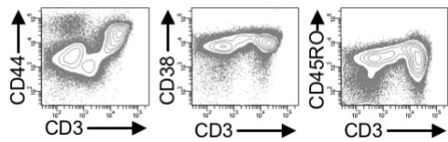
Suppl. Fig. 1. CD44 expression is highest and CD38 and CD45RO are lowest at the CD3 lo developmental stage. Total thymocytes were labeled with CD44, CD38, CD45RO, and CD3 and analyzed by flow cytometry.
