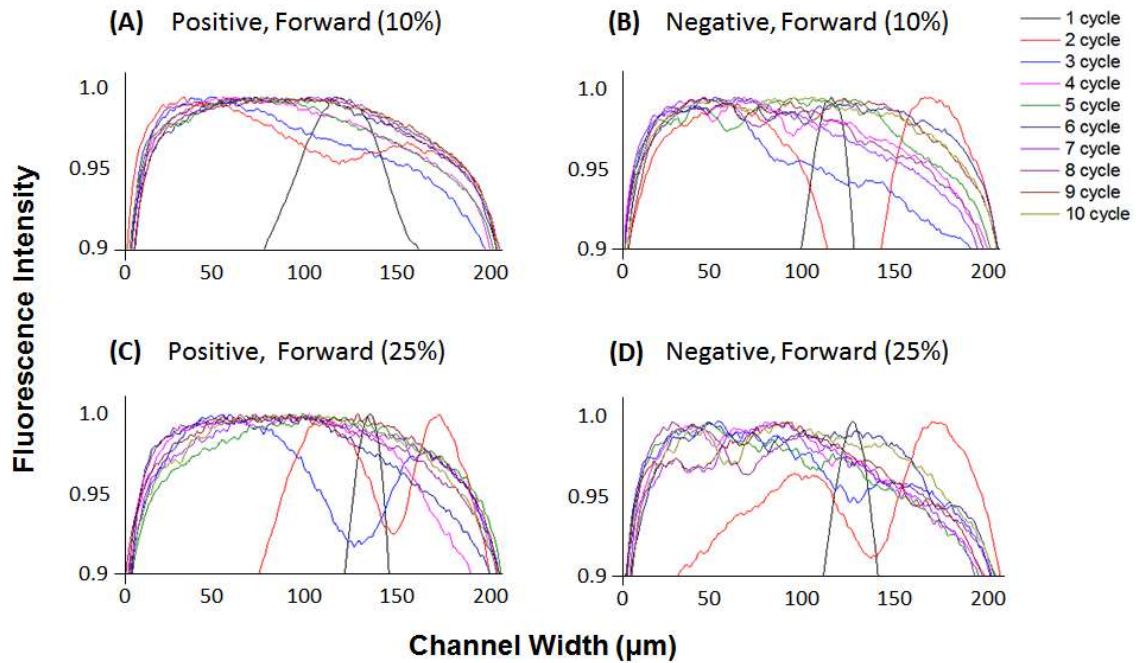
S4 Fig. Normalized fluorescence intensity across the microchannel in viscous fluid test. After each cycle from 1 to 10. (A) 10% Positive forward, (B) 10% Negative forward, (C) 25% Positive forward, (D) 25% Negative forward.
