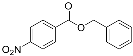
benzyl 4-nitrobenzoate
