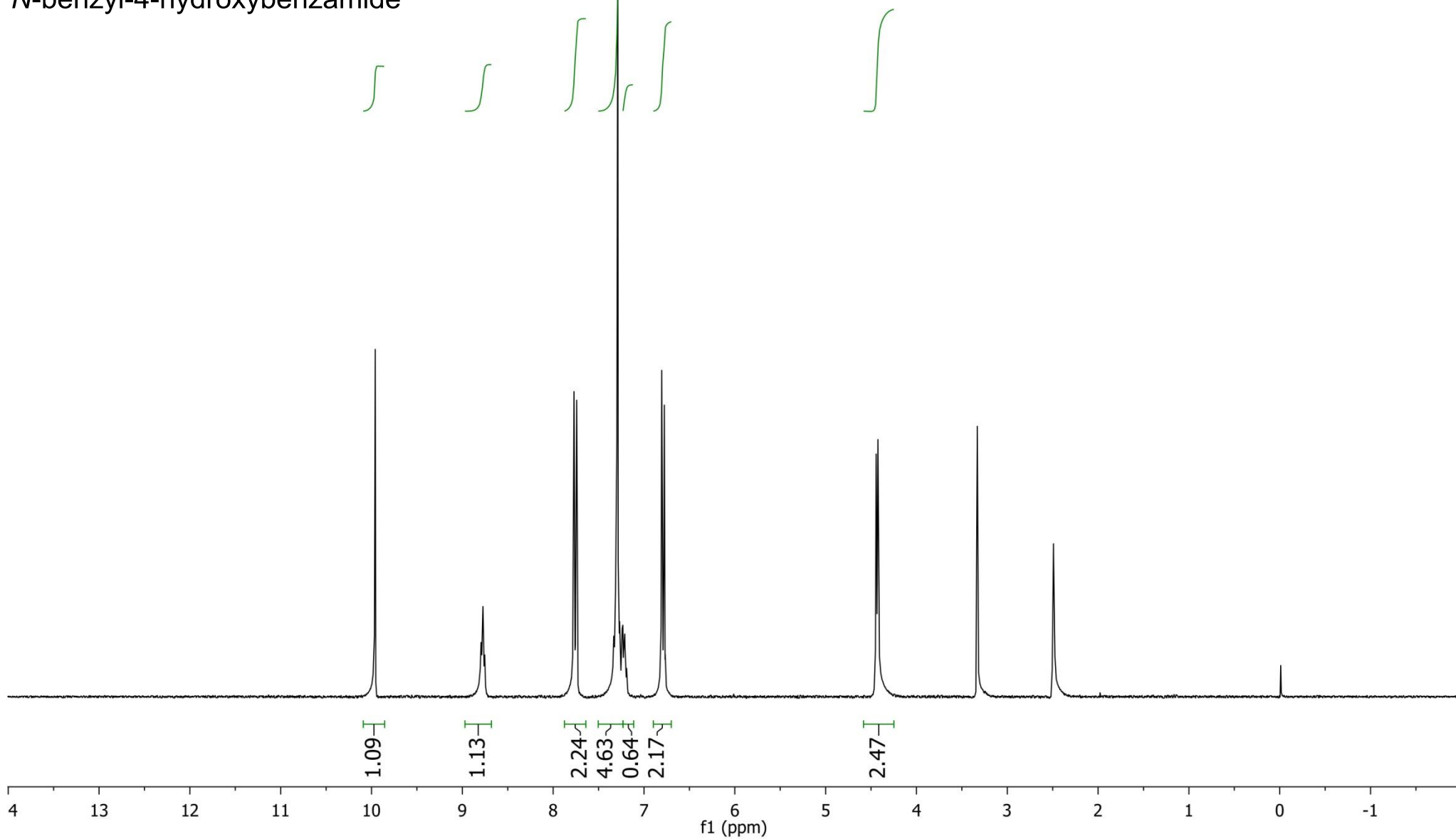
N -benzyl-4-hydroxybenzamide
