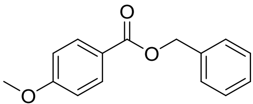
benzyl 4-methoxybenzoate
