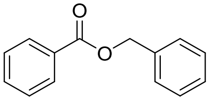
benzyl benzoate
