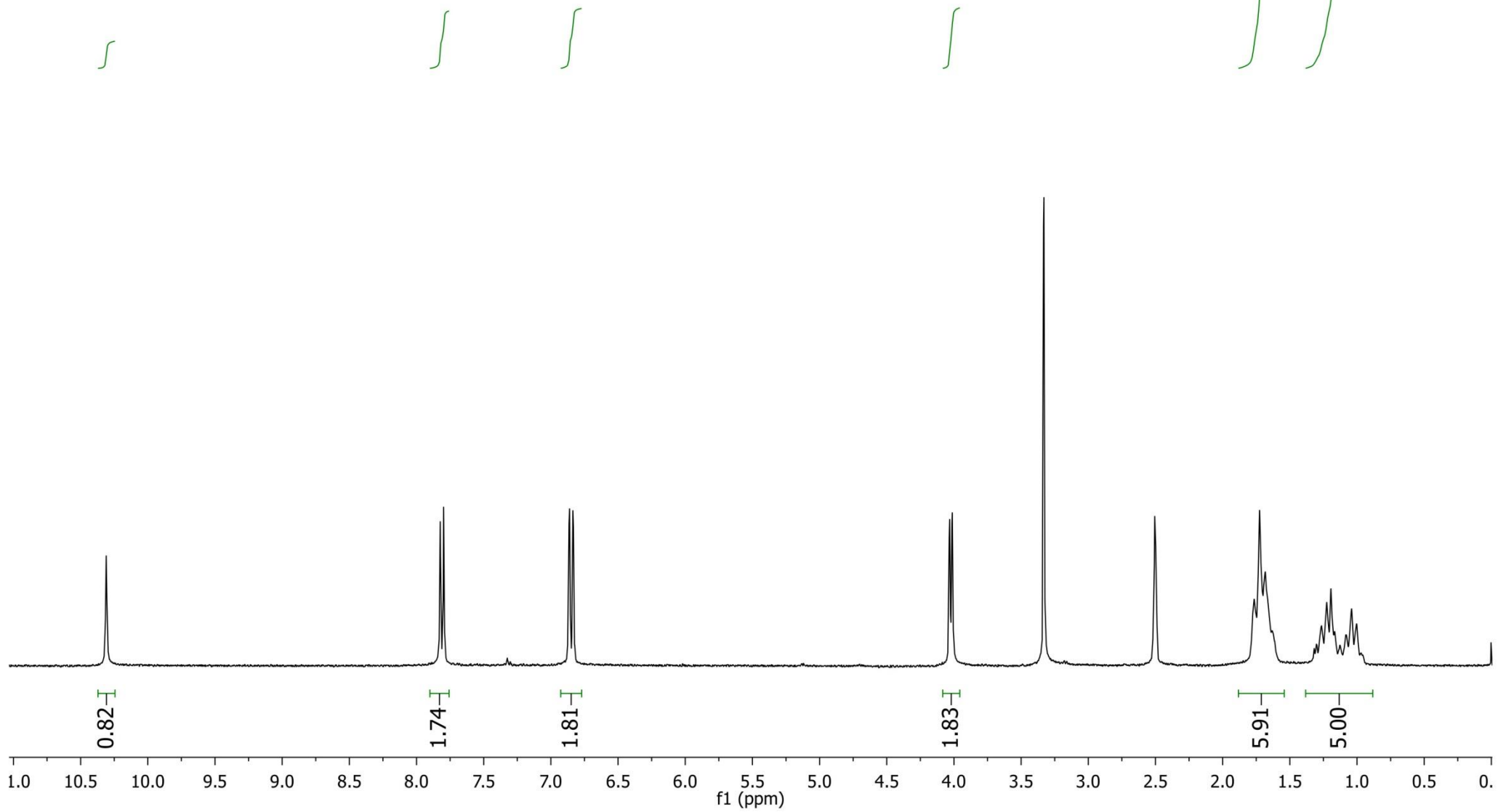
cyclohexylmethyl 4-hydroxybenzoate
