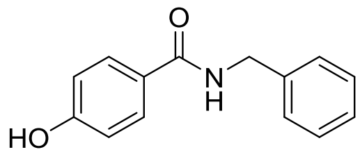
N -benzyl-4-hydroxybenzamide
