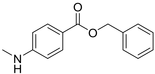
benzyl 4-(methylamino)benzoate
