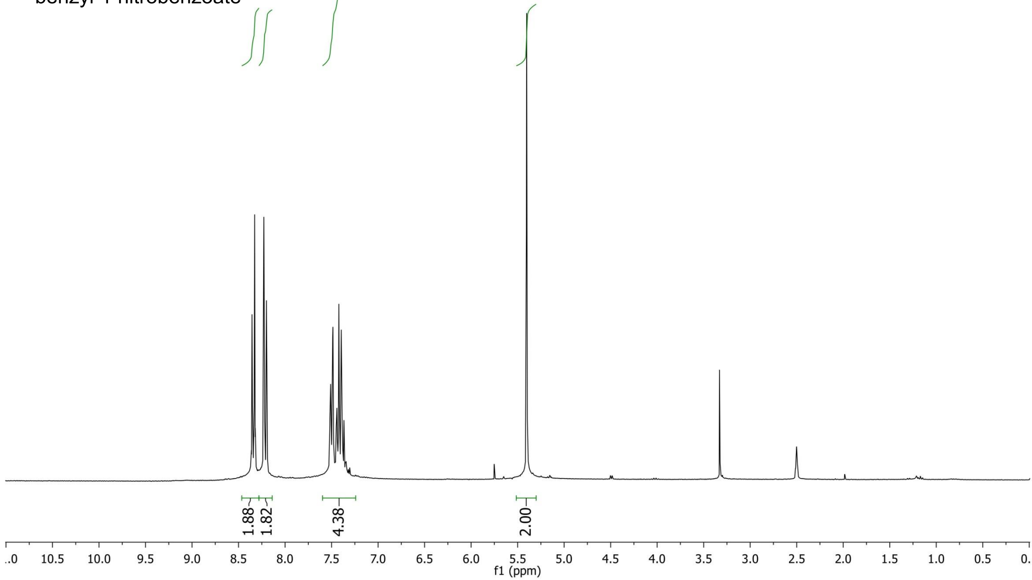
benzyl 4-nitrobenzoate
