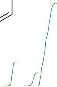
benzyl benzoate
