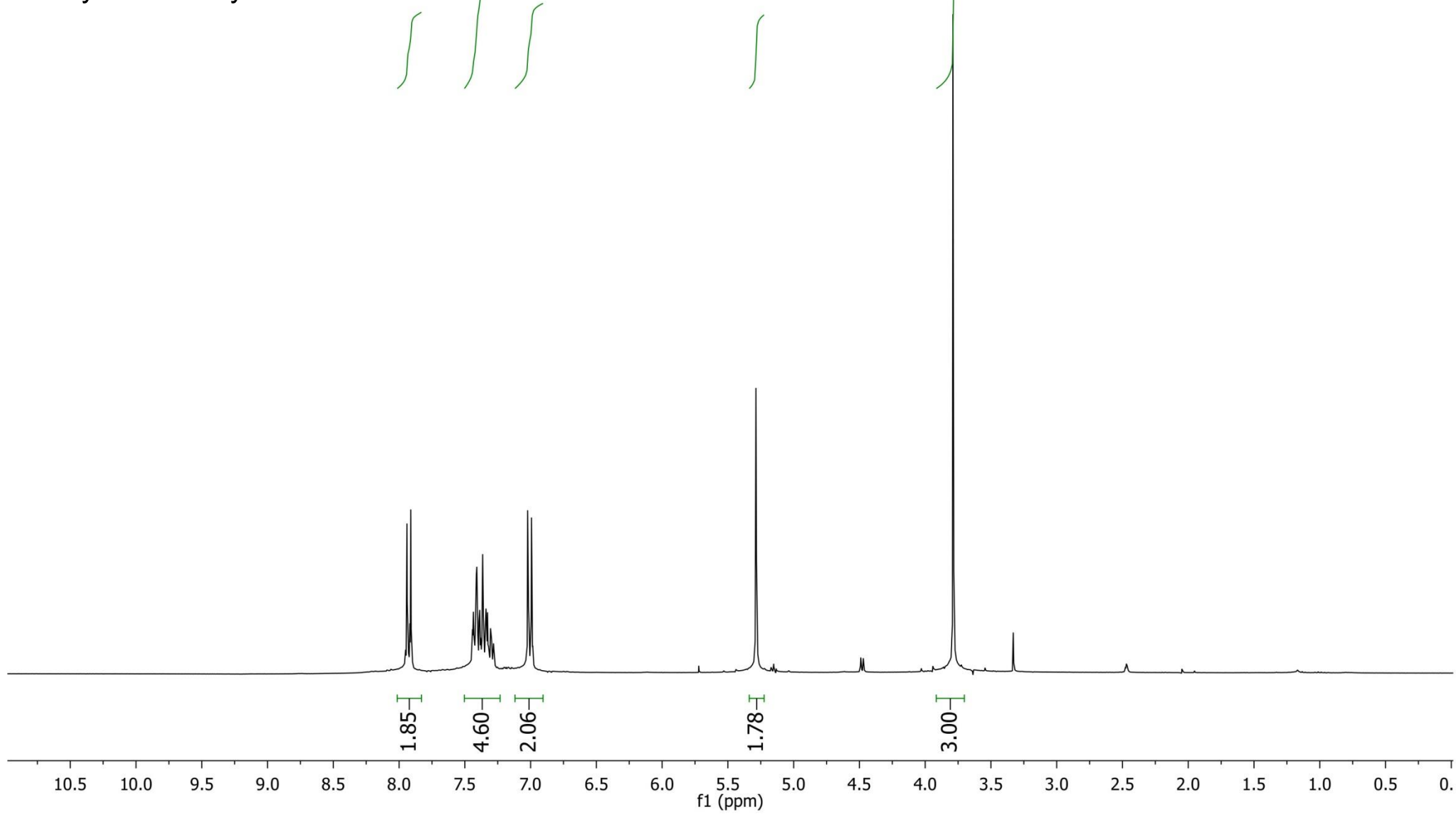
benzyl 4-methoxybenzoate
