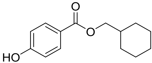
cyclohexylmethyl 4-hydroxybenzoate
