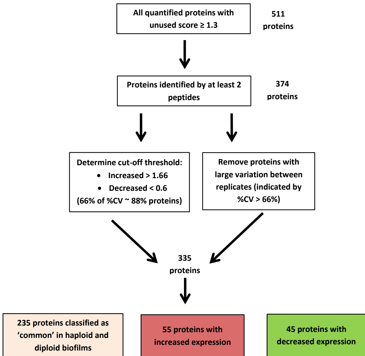
Figure S1. Flow chart illustrating the different filtering methodology used to analyse the differentially expressed proteins among biofilm samples of haploid and diploid Candida albicans .
