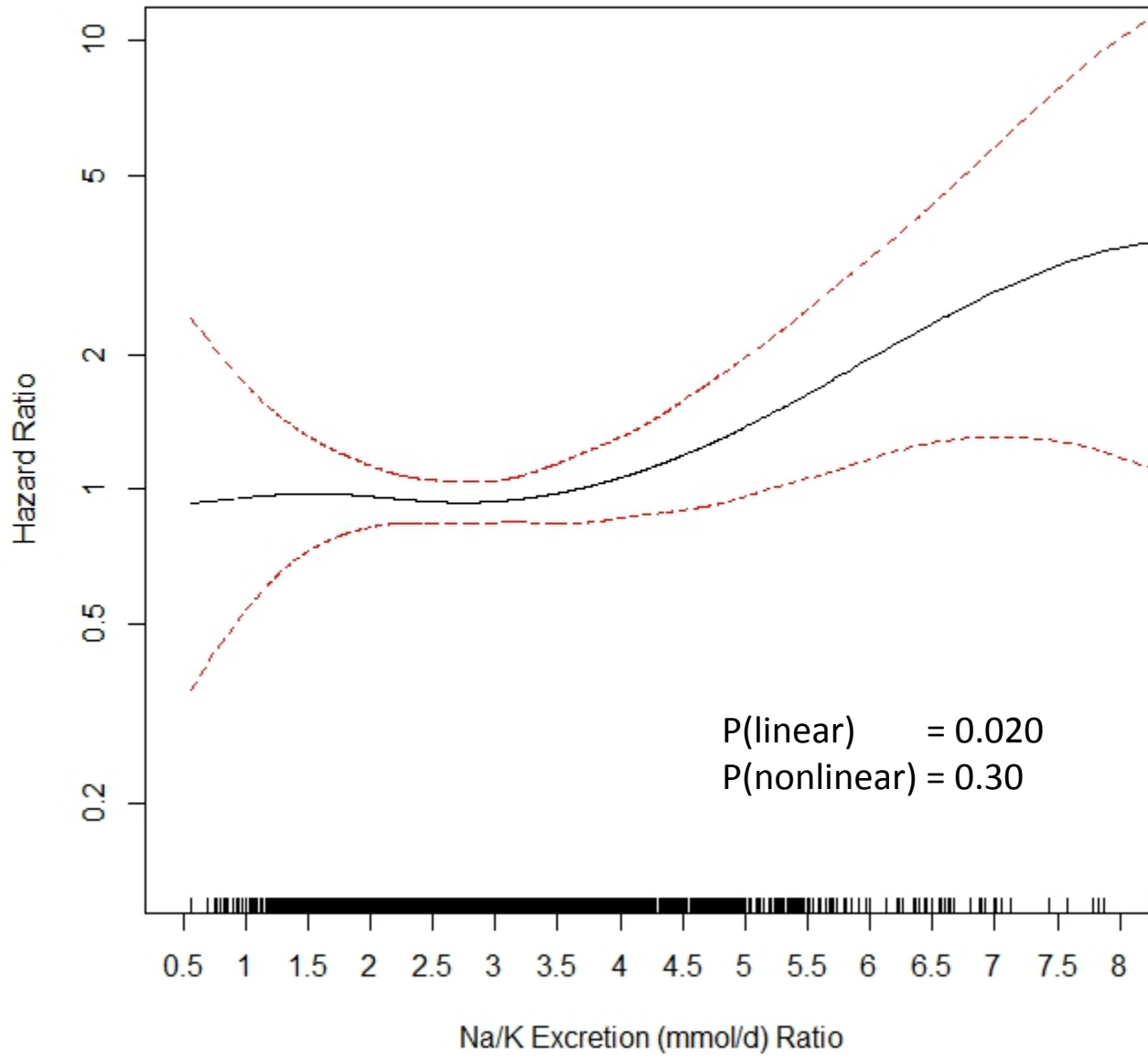
Spline Plot of Sodium/Potassium Ratio and Total Mortality
