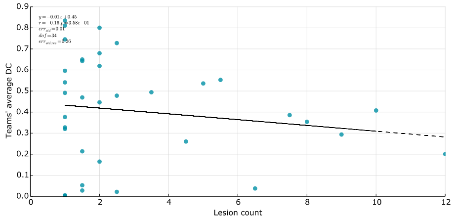
Figure 2: Correlation between the number of lesions and average DC over all teams per case.
