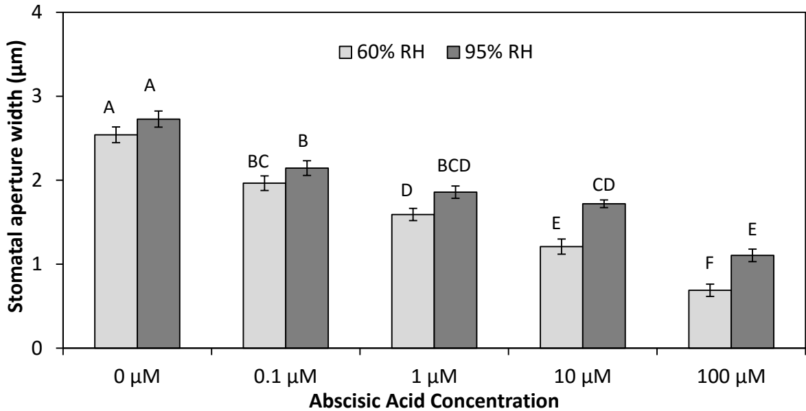
Figure S3. Addition of exogenous abscisic acid is not enough to completely close the stomatal pore under high relative humidity (RH). Stomatal aperture width in intact leaves of Col-0 2 h after exposure to the varying concentrations of abscisic acid. Data points are average ( n > 60 ) \pm SE and different letters above the bars indicate statistical significance ( p < 0.05 ) calculated with ANOVA.
