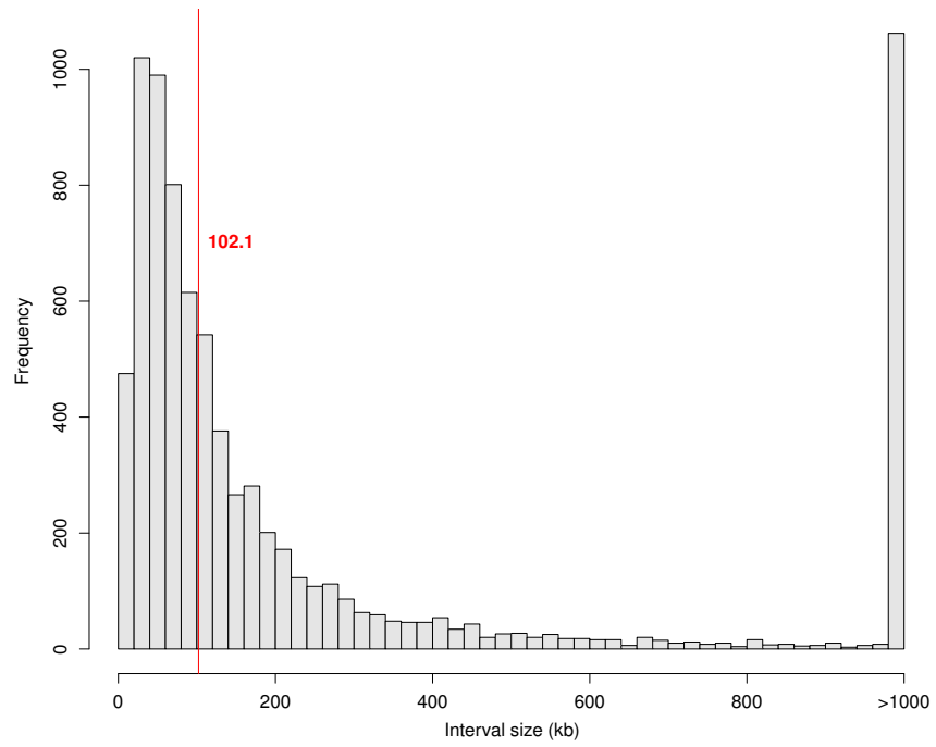
Figure S7: Distribution of crossover interval size. The vertical red line represents the median interval size of 102.1 kb.
